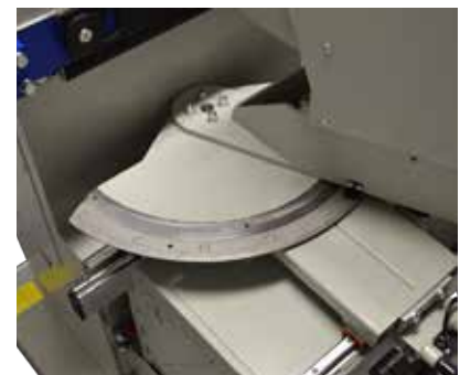
Bohraggregat schwenkbar -65° - 0 - 65°
